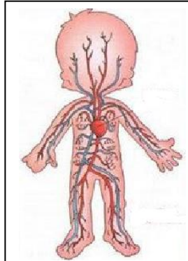
Aparell circulatori
