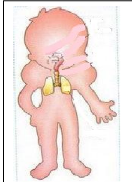
Aparell respiratori
